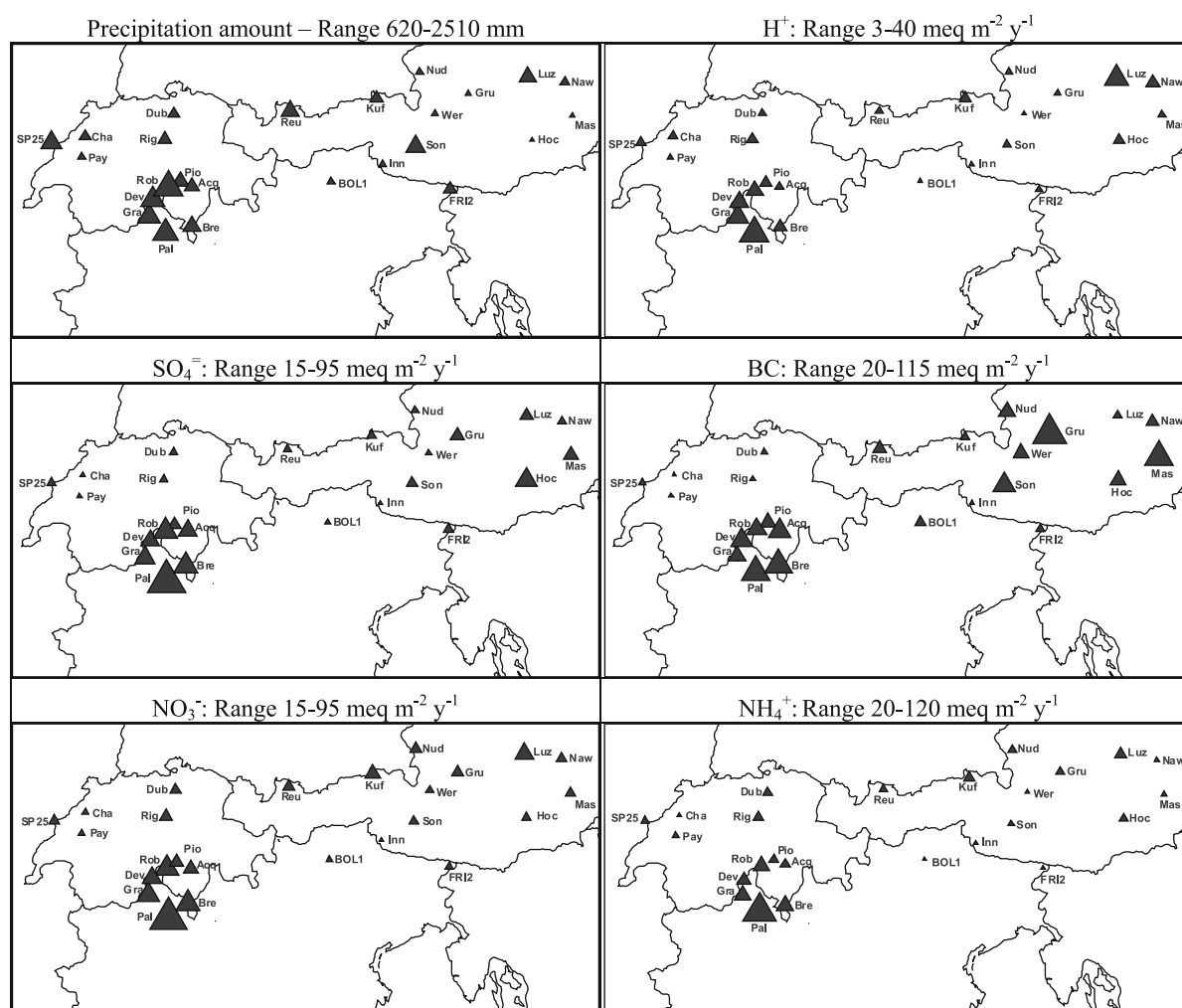
Figure 3. Precipitation amount and fluxes of H^+ , SO_4^{2-} , BC (base cations = Ca^{++} + Mg^{++} + Na^+ + K^+ ), NO_3^- and NH_4^+ at wet-only sampling sites (volume weighted mean of 1998–2002). Triangles are proportionally scaled to deposition values. Acronyms as in Table 1.
