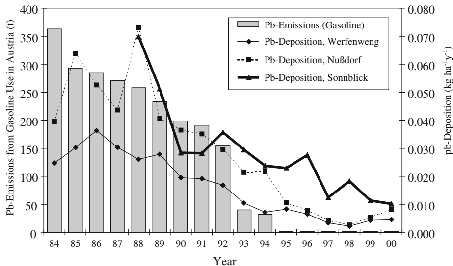
Figure 6. Lead deposition at three sites in Austria compared to lead emissions from gasoline in the period 1984–2000.
