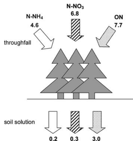
Figure 5. Results of the nitrogen mass balance at the forested site LOM1, Val Masino, Northern Italy. Units: \text{kg ha}^{-1} \text{ y}^{-1} .
